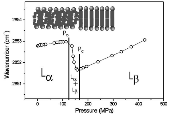
Fig. 1. Main phase transition of POPC at 25 °C at full hydration (RH = 100%), detected by using the symmetric stretching vibrations, \nu_{sym}(\text{CH}_2) , depending on hydrostatic pressure. The coexistence region between liquid crystalline ( L_\alpha ) and gel-phase ( L_\beta ) starts at the onset pressure P_0 and stops at the completion pressure P_c .
